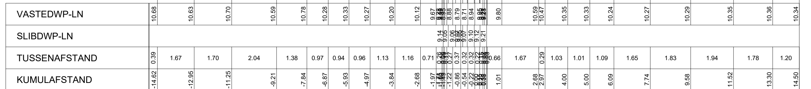
Km 5363.75m Hsch 1/100 Lsch 1/100 Vvlak 0.00 T.A.W.
