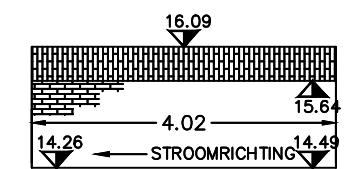
K400 LANGSDOORSNEDE
