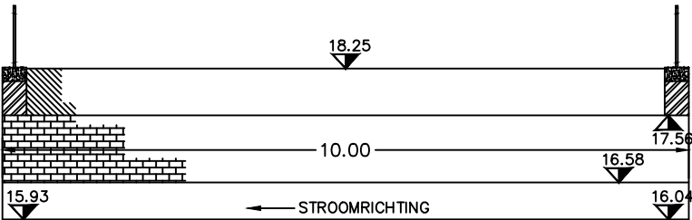
K460 LANGSDOORSNEDE
